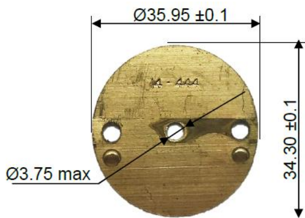
REF.26 - P. N° 14-A127 THROTTLE SHUTTER
